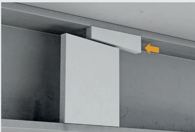
Wedged nogging
