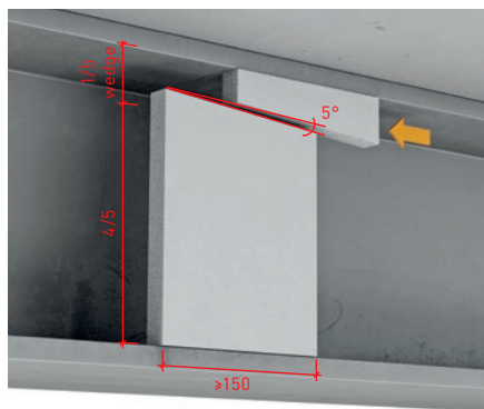
Detail option for single-layer nogging
