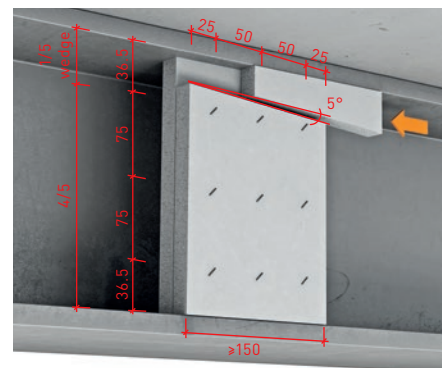
Detail option for dual-layer nogging
