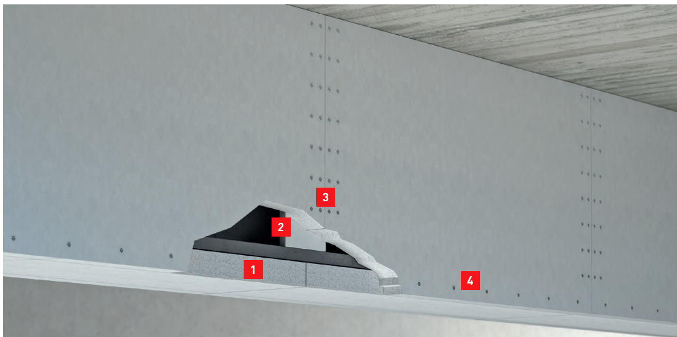
Beam with cladding on three sides
